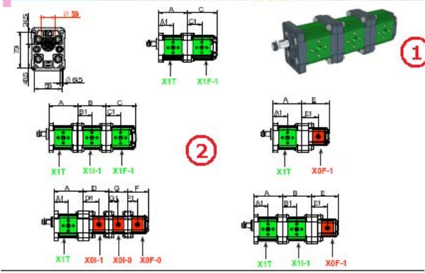
POMPA MULTIPLA XV-1 BASE # 30
